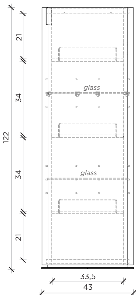
FRONTE | FRONT
