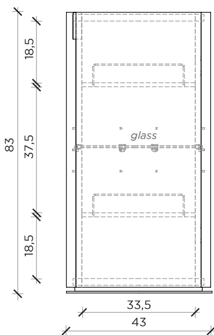
FRONTE | FRONT
