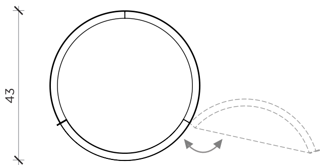
FRONTE | FRONT
