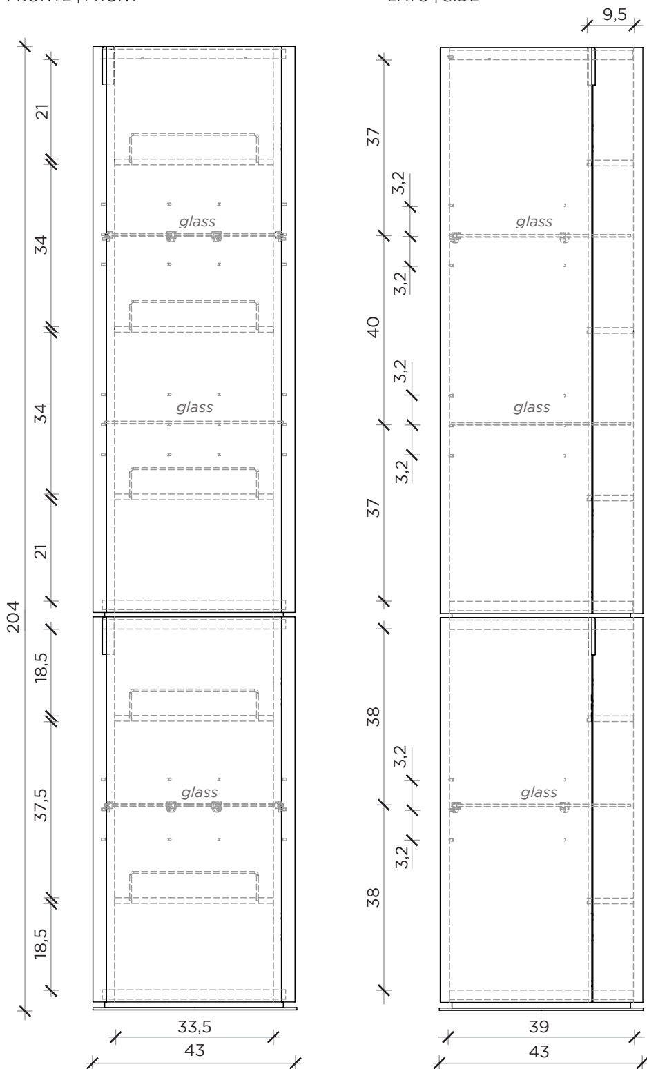
FRONTE | FRONT
